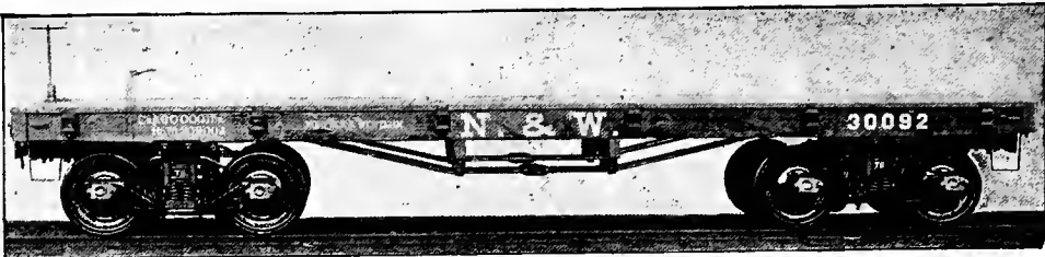
Fig. 17. FLAT CAR NORFOLK & WESTERN RAILROAD. Length, 34 ft. Capacity, 60,000 lbs. Weight, 20,900 lbs. Equipped with Rigid Diamond Trucks.
